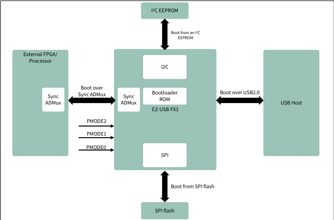
Figure 1 FX3 启动选项
