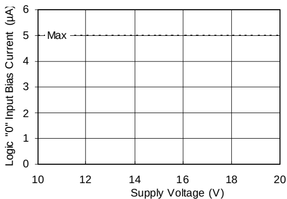
Figure 13B. Logic "0" Input Bias Current vs. Voltage
