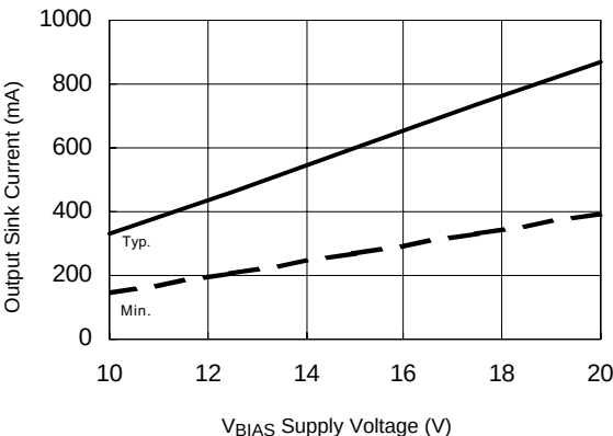
Figure 23B. Output Sink Current vs. Supply Voltage
