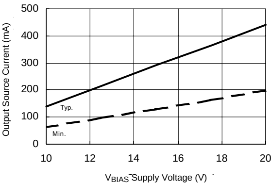
Figure 22B. Output Source Current vs. Supply Voltage
