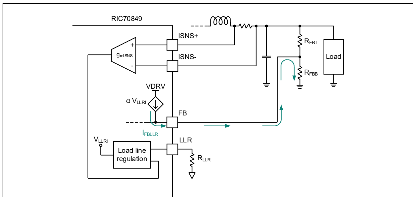
Figure 30 Simplified schematic of LLR operation in RIC70849
