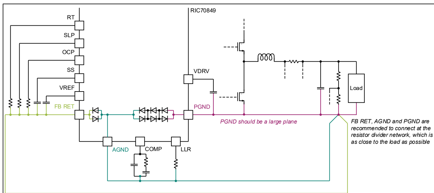
Figure 22 Example external connections for return pins PGND, AGND and FB RET
