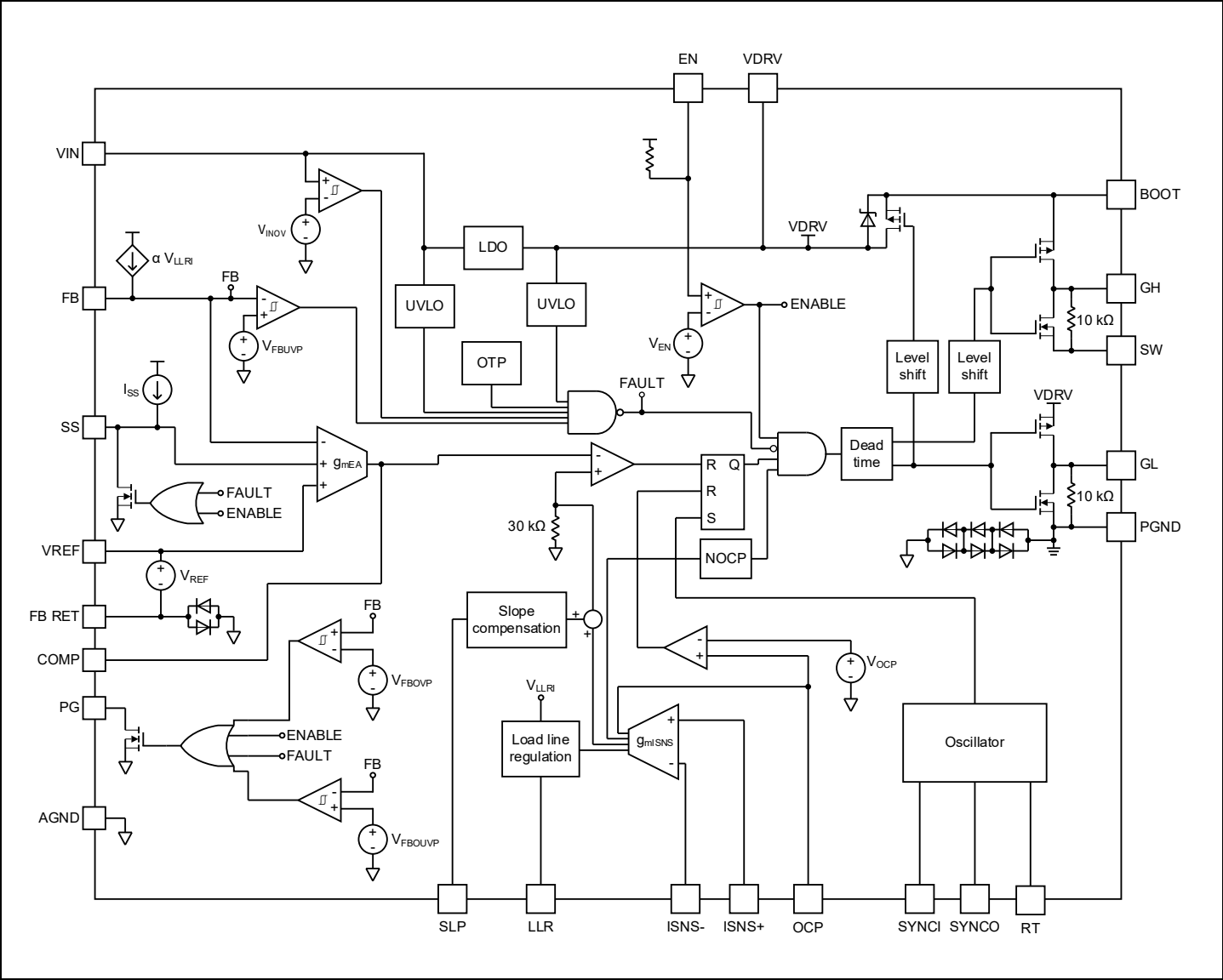
Figure 2 RIC70849 block diagram
