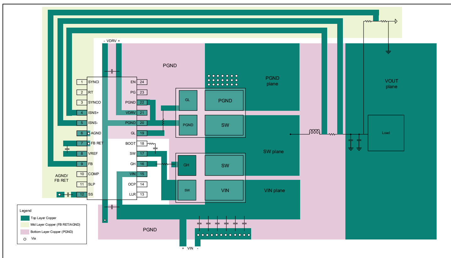
Figure 34 Recommended PCB layout for RIC70849
