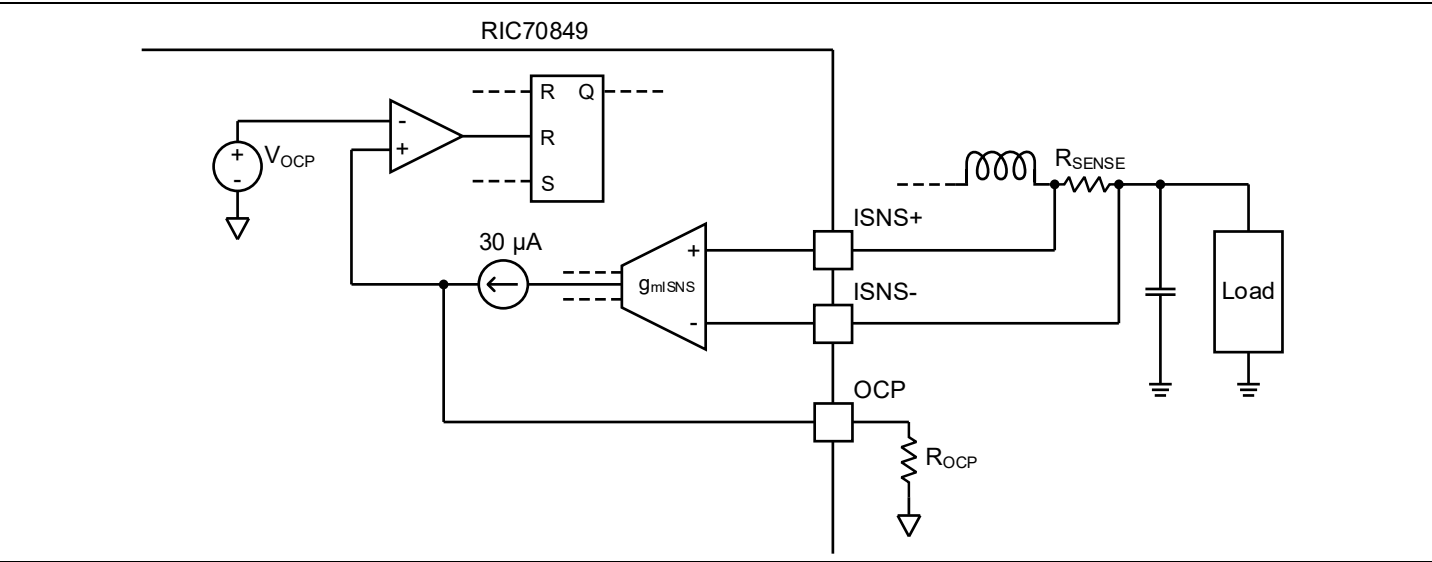
Figure 31 Simplified schematic of RIC70849 overcurrent protection with current sense resistor, with offset current of 30 \mu\text{A} shown externally for clarity
