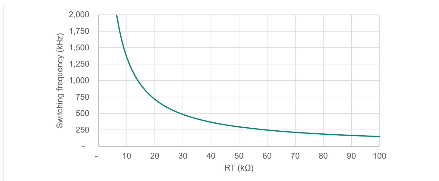
Figure 24 Switching frequency vs. resistor on RT pin
