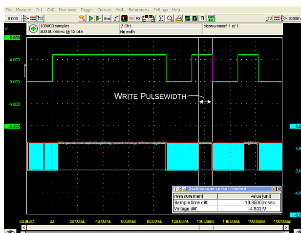
Figure 4. Measuring the Write Pulse Width
