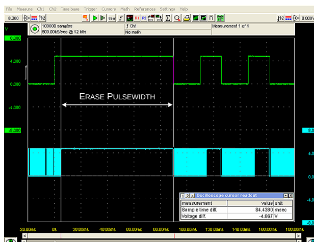
Figure 3. Measuring the Erase Pulse Width
