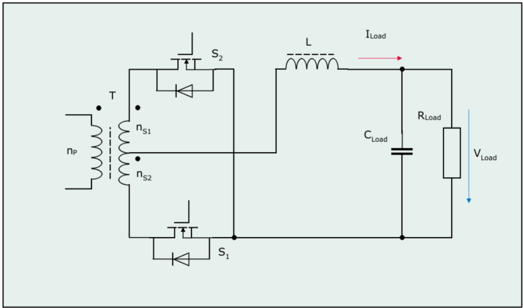
› Full wave rectifier
